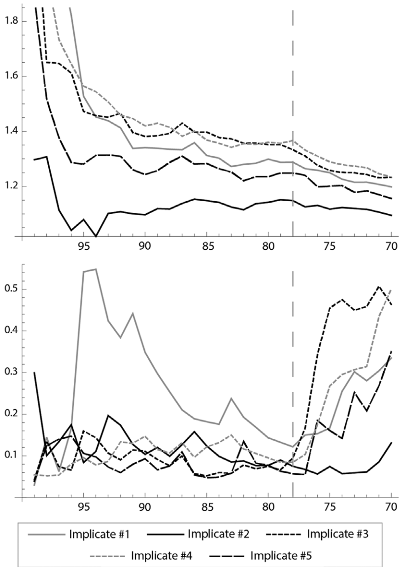
Figure 4. Estimates for Pareto's \alpha and Corresponding Cramer von Mises Test Statistics Across All Implicates
